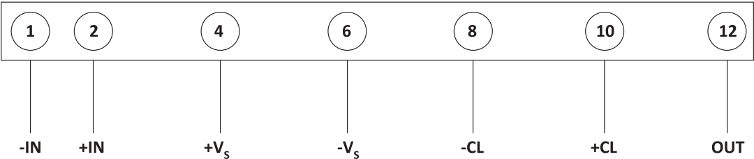
Figure 3: External Connections
