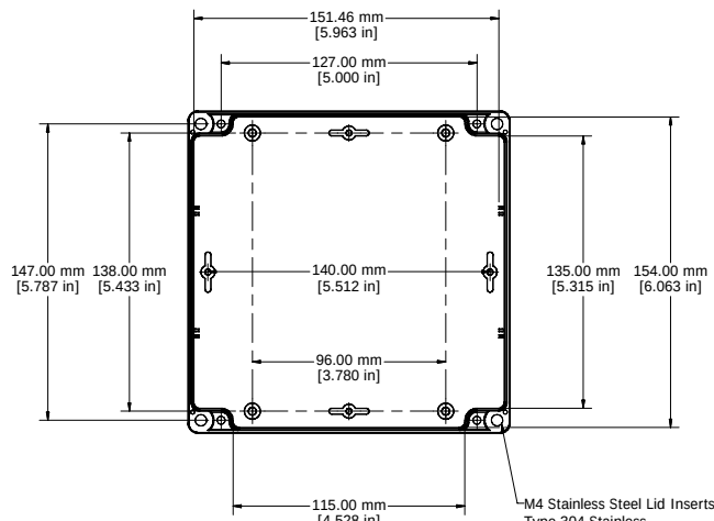
BOX - INSIDE
