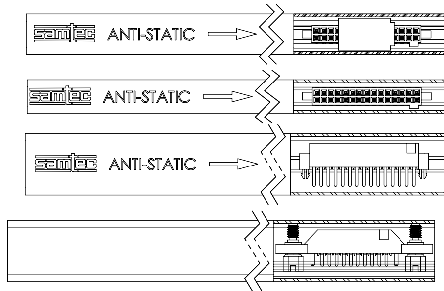
PACKAGING VIEW PACKAGE PARTS IN TUBES AS SHOWN (SEE NOTE 4)
