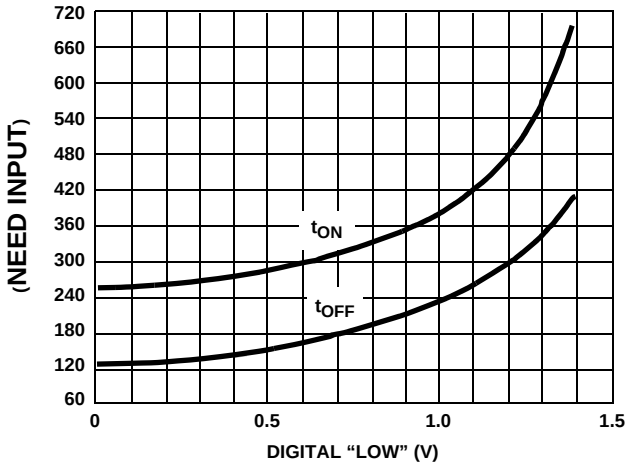
FIGURE 7F. SWITCHING TIMES vs NEGATIVE DIGITAL VOLTAGE
