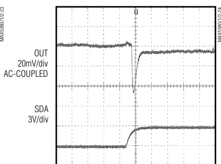
OUTPUT SETTLING 1LSB STEP DOWN
