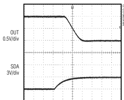
OUTPUT SETTLING FROM 3/4 FS TO 1/4 FS
