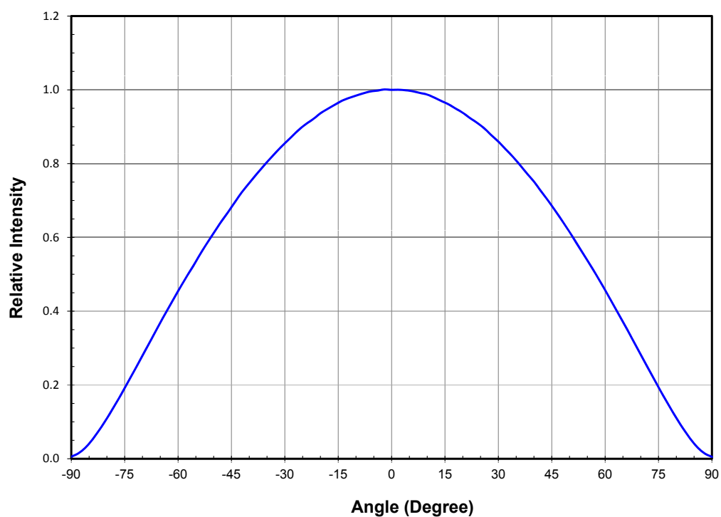
Figure 10. Typical representative spatial radiation pattern.
