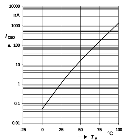
Dark Current
