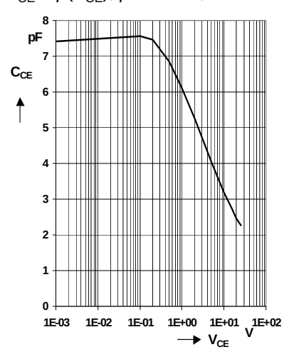
Collector-Emitter Capacitance
