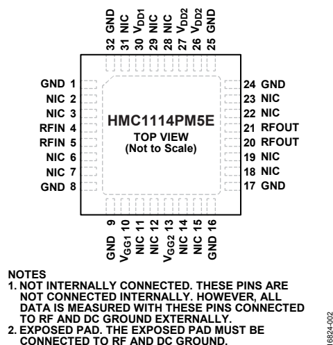
Figure 2. Pin Configuration
