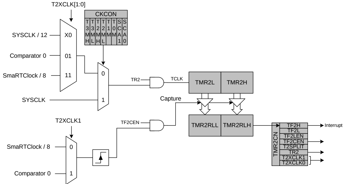
Figure 32.6. Timer 2 Capture Mode Block Diagram
