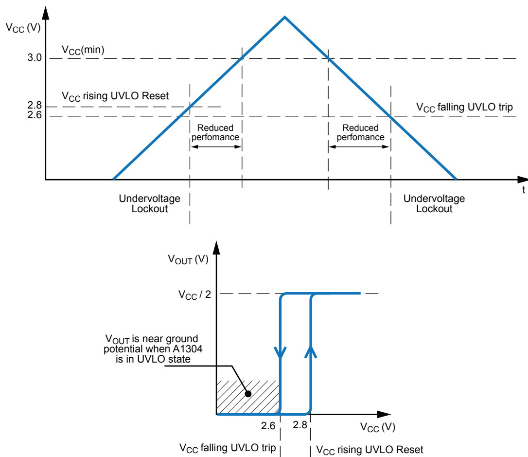
Figure 4: UVLO Operation
