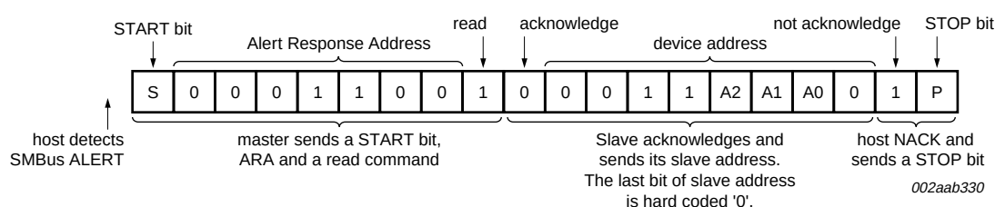
Fig 6. How SE98 responds to SMBus Alert
