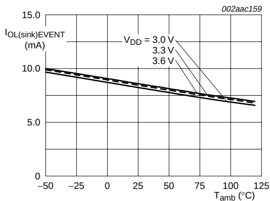
Fig 16. \overline{\text{EVENT}} sink current at 0.4 V versus temperature
