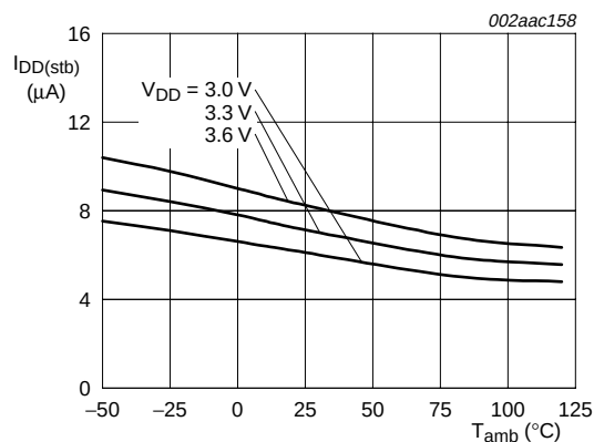
Fig 15. Standby supply current versus temperature
