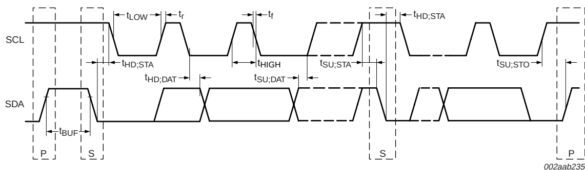
Fig 19. AC timing diagram
