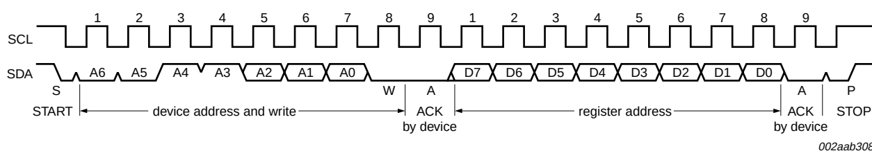
Fig 7. SMBus/I 2 C-bus write to the Pointer register
