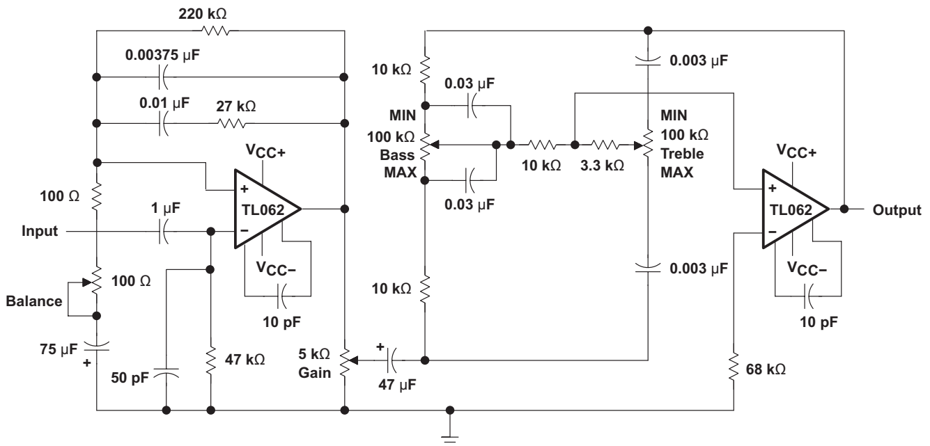
Figure 27. IC Preamplifier
