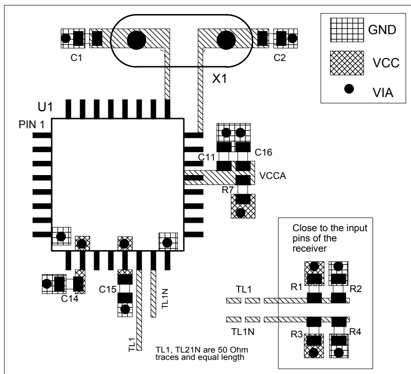
FIGURE 7B. PCB BOARD LAYOUT FOR ICS8430-61
