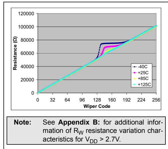
FIGURE 2-75: 100 kΩ – R_{WB} ( \Omega ) vs. Wiper Setting and Ambient Temperature ( V_{DD} = 1.8\text{V} , I_W = 15\text{ }\mu\text{A} ).
