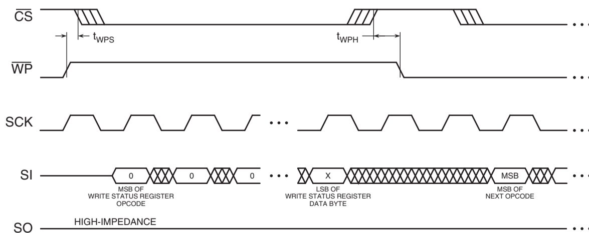
Figure 13-5. \overline{\text{WP}} Timing for Write Status Register Command When SPRL = 1
