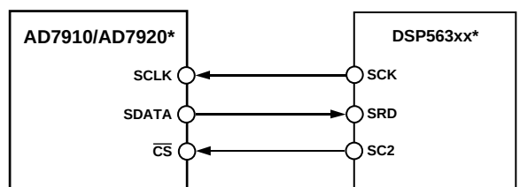
Figure 27. Interfacing to the DSP563xx
