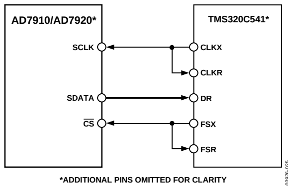
Figure 25. Interfacing to the TMS320C541
