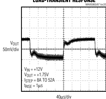
LOAD-TRANSIENT RESPONSE
