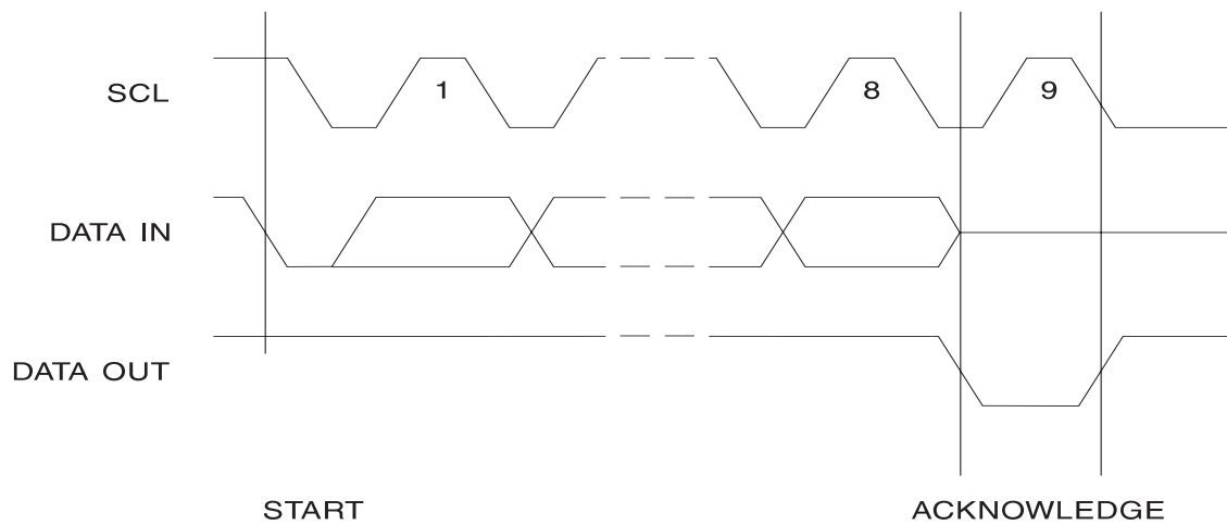
Figure 6. Output Acknowledge
