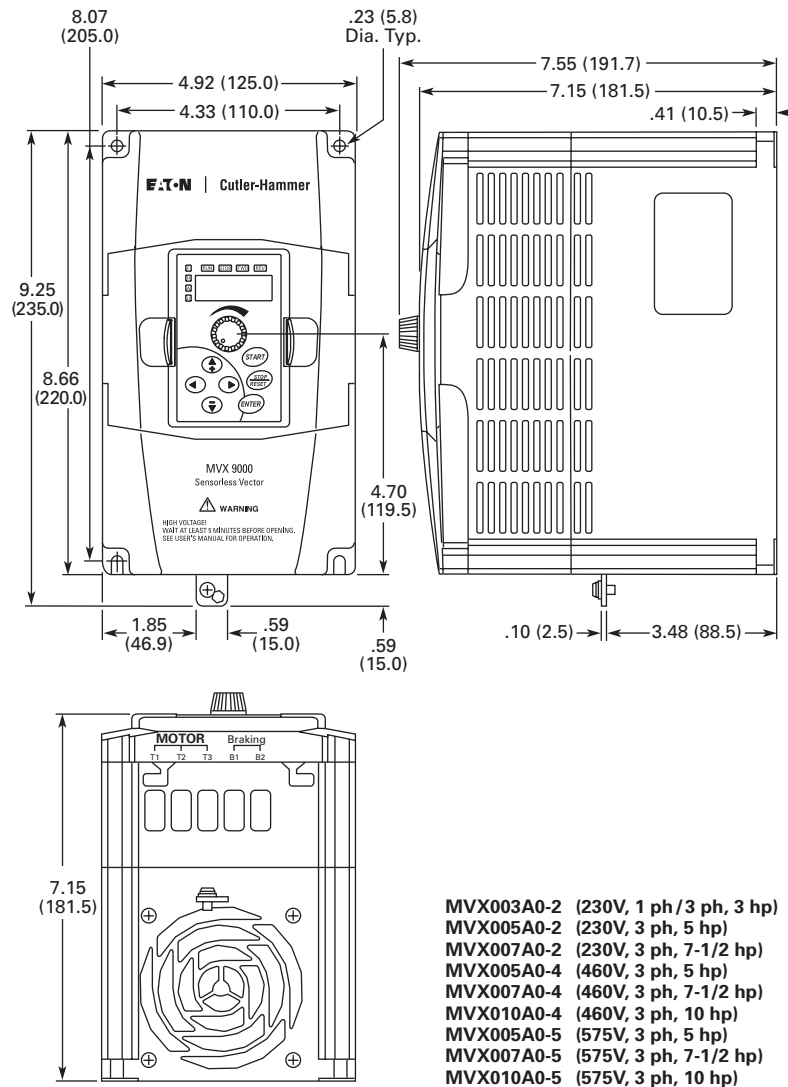
Figure 4. 3 to 10 hp Drive Approximate Dimensions in Inches (mm)
