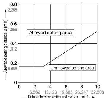
<Side mounting>
