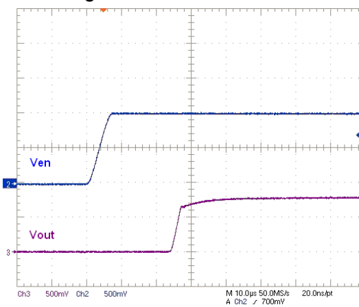
Figure 13. Enable transient
