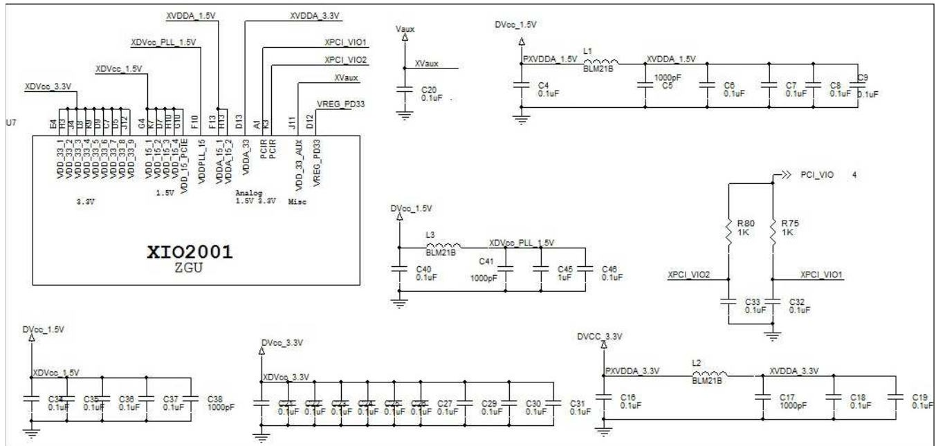
Figure 31. Power Filtering
