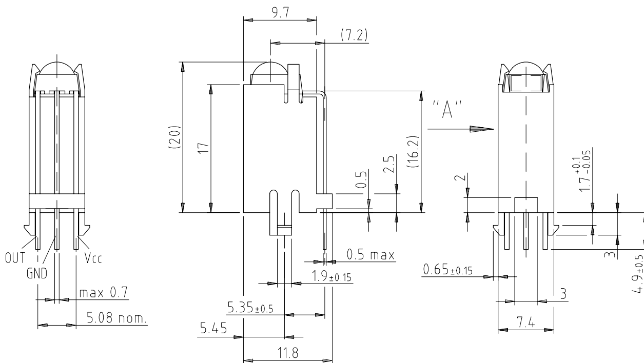
View "A"
