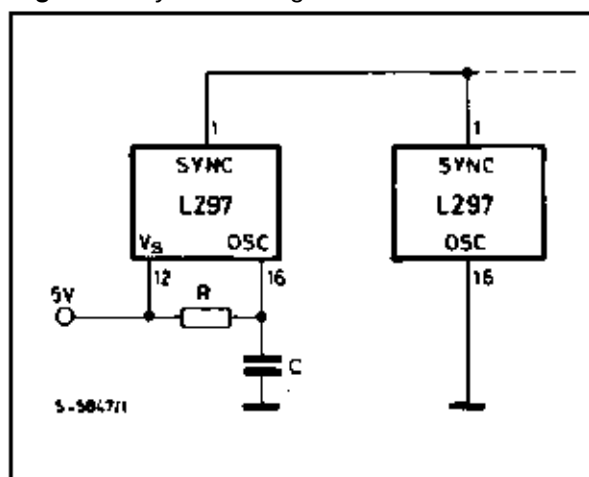
Figure 3 : Synchronising L297s
