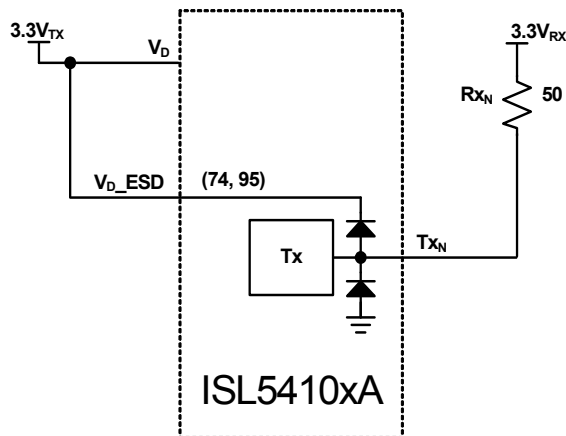
FIGURE 10. ISL5410xA ESD PROTECTION DIODES
