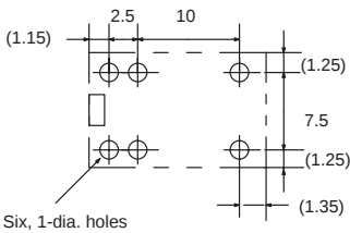
Mounting Holes (Bottom View) Tolerance: ±0.1
