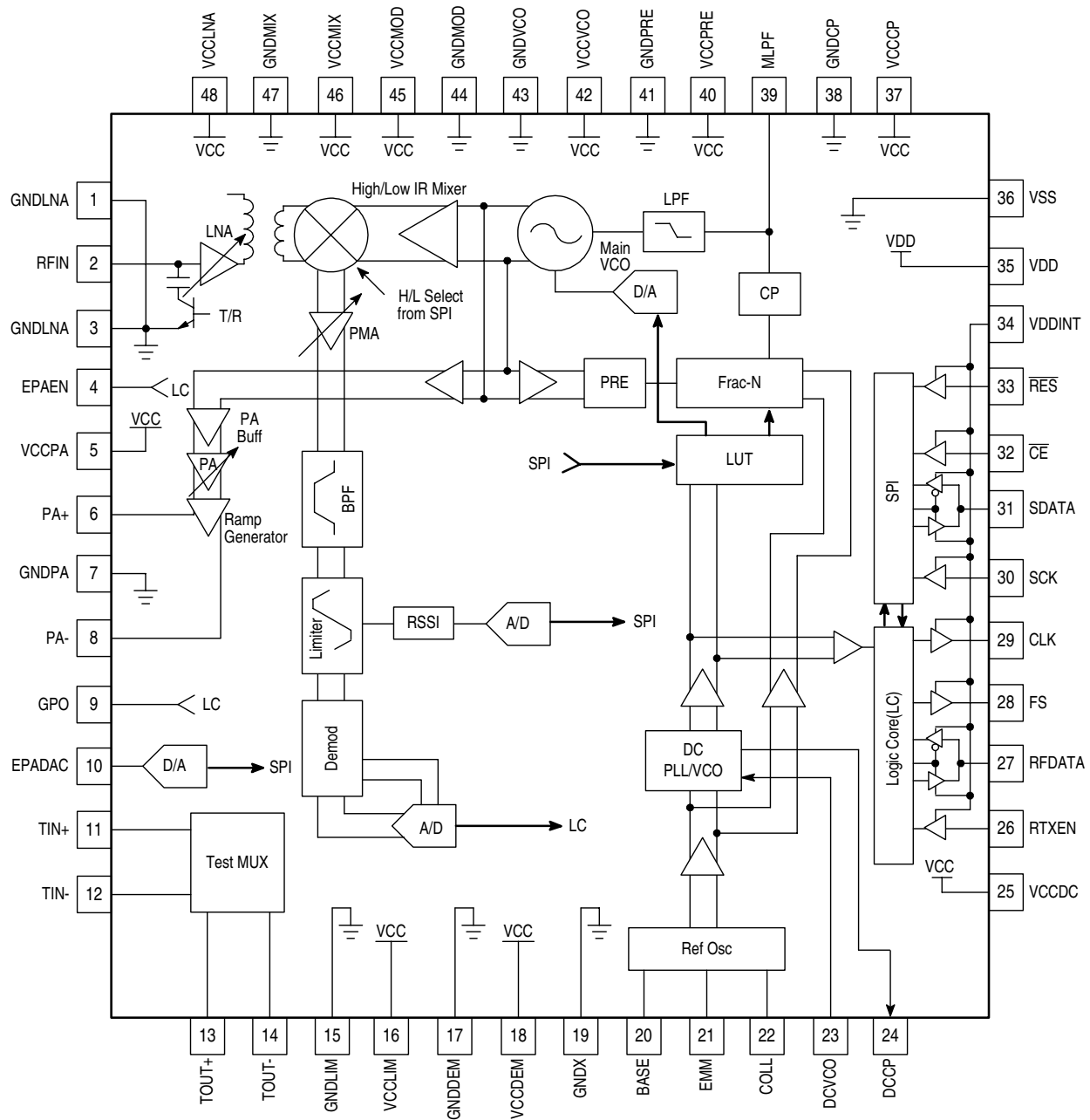
Figure 2. Device Pinout
