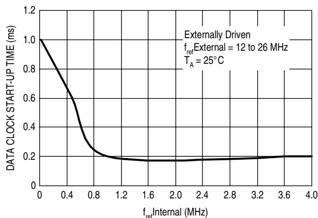
Figure 21. Data Clock Start-up Time versus f_{\text{refInternal}}
