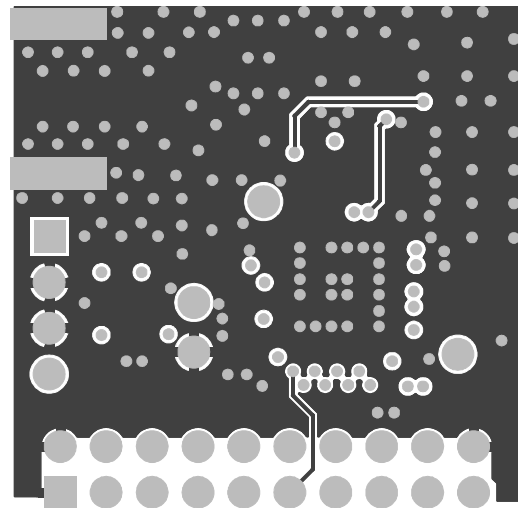
Figure 47. Bottom Plane
