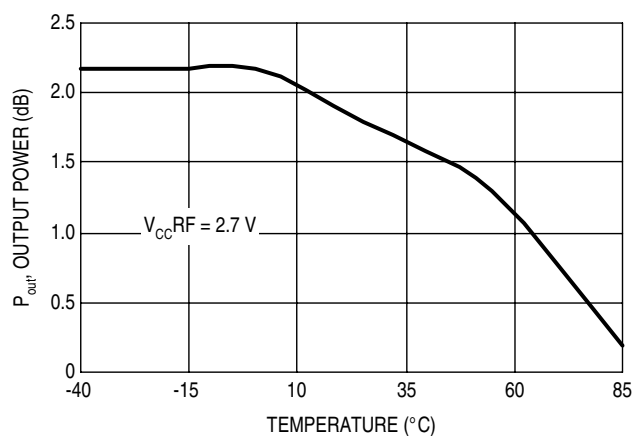
Figure 36. RF Output Power versus Temperature
