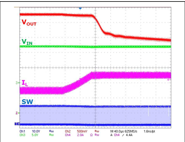
Figure 16. Overcurrent protection
