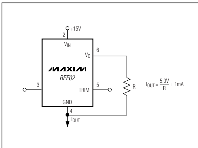
Figure 4. Current Source
