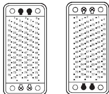
Plug Receptacle
