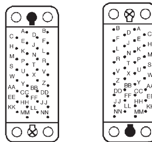
75-way
