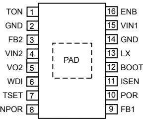
LP-16 PINOUT DIAGRAM
