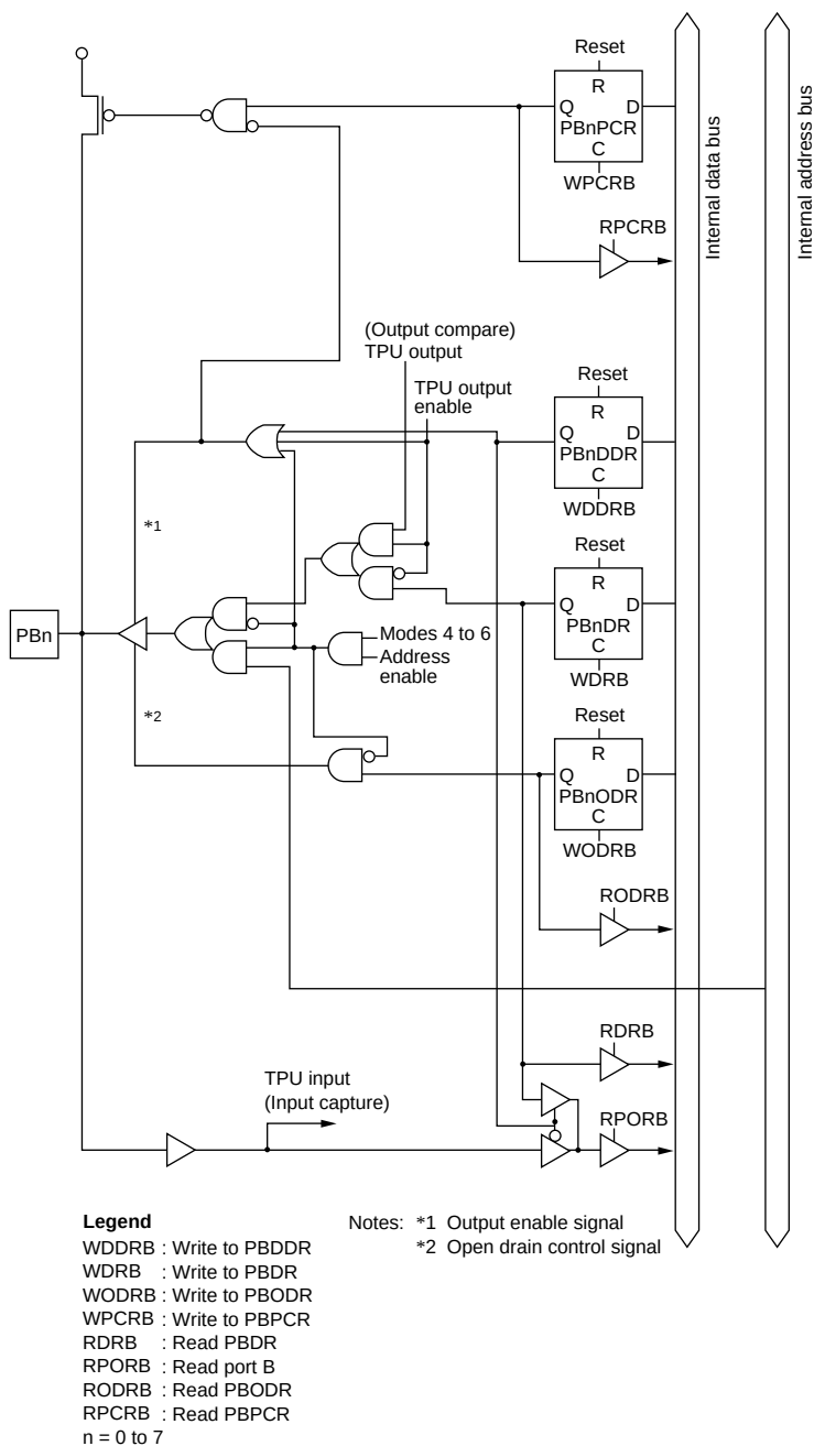
Figure C-19 Port B Block Diagram (Pins PB0 to PB7)
