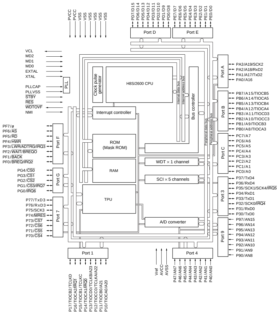
Figure 1-1 (c) H8S/2695 Internal Block Diagram
