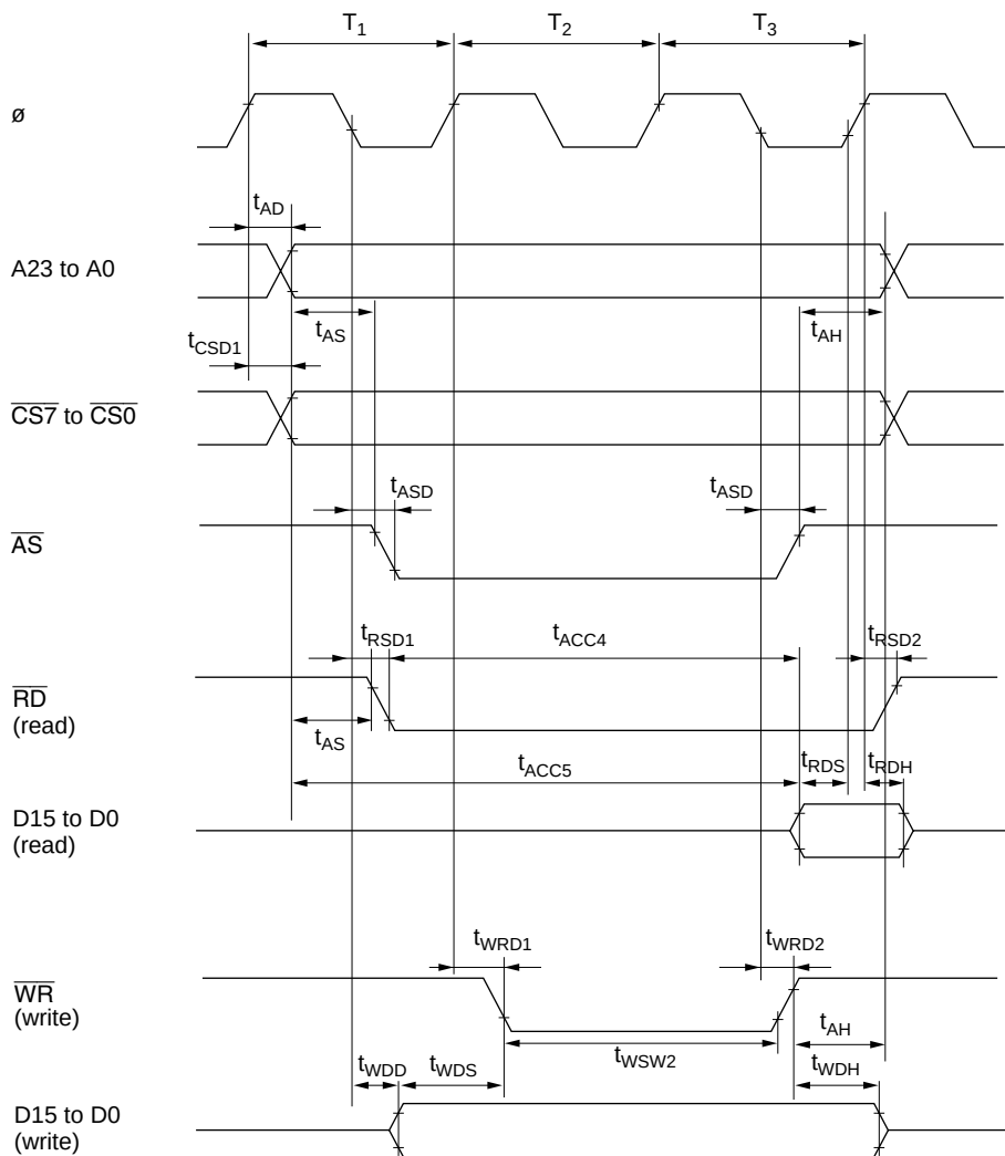
Figure 26-7 Basic Bus Timing (Three-State Access)
