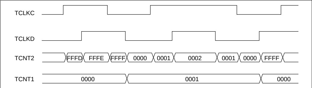
Figure 11-23 Example of Cascaded Operation (2)
