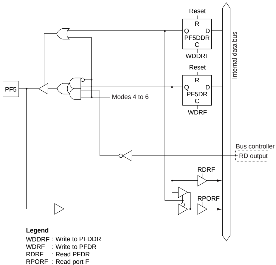
Figure C-23 (f) Port F Block Diagram (Pin PF5)
