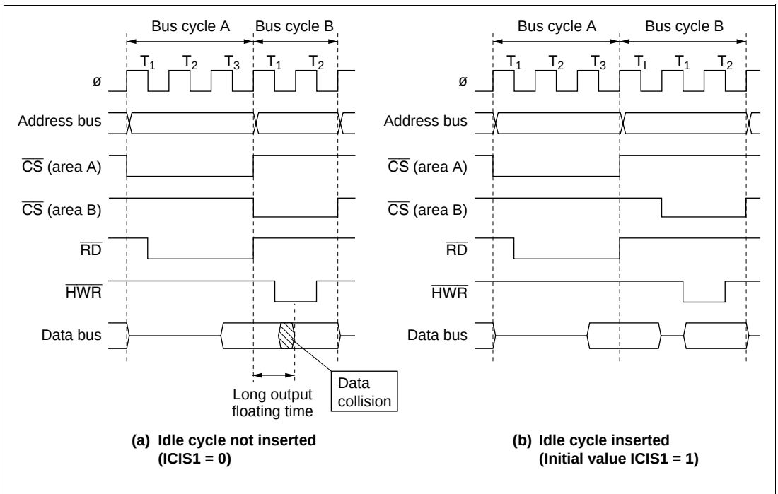
Figure 7-35 Relationship between Chip Select ( \overline{\text{CS}} ) and Read ( \overline{\text{RD}} )
