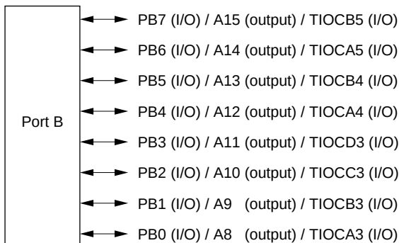
Figure 10A-10 Port B Pin Functions (Modes 4 to 6)
