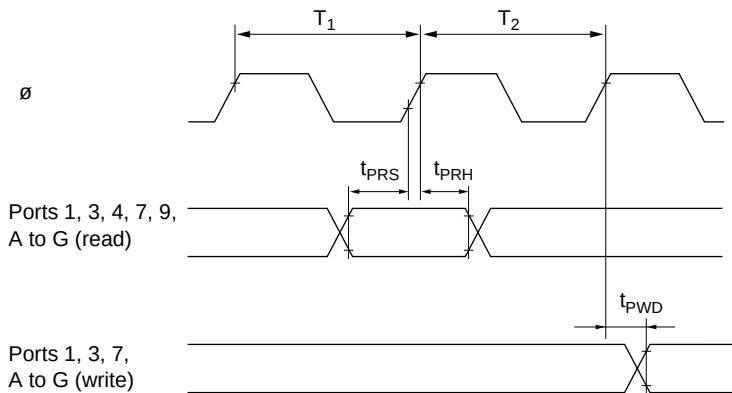
Figure 27-13 I/O Port Input/Output Timing
