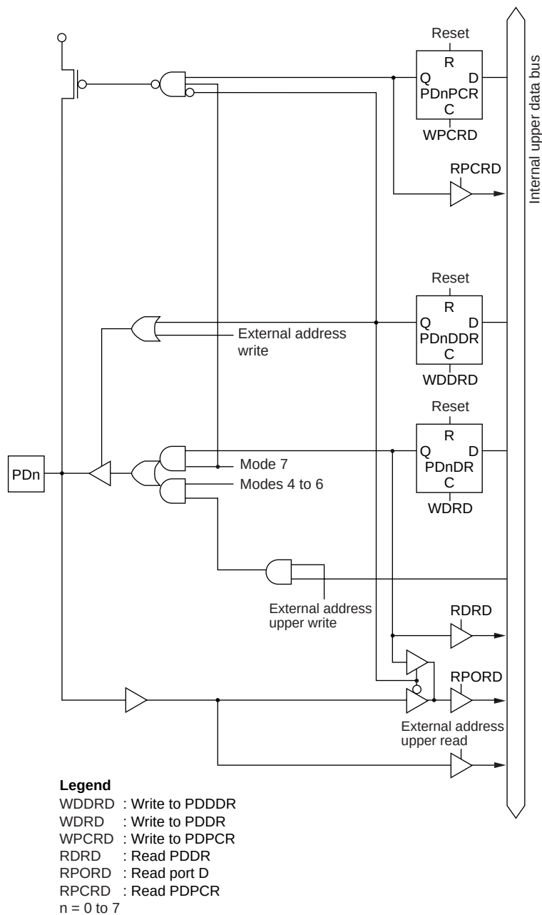
Figure C-21 Port D Block Diagram (Pins PD0 to PD7)
