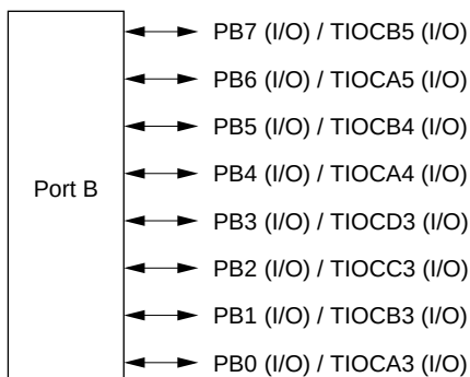
Figure 10A-11 Port B Pin Functions (Mode 7)
