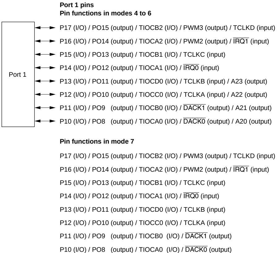
Figure 10A-1 Port 1 Pin Functions
