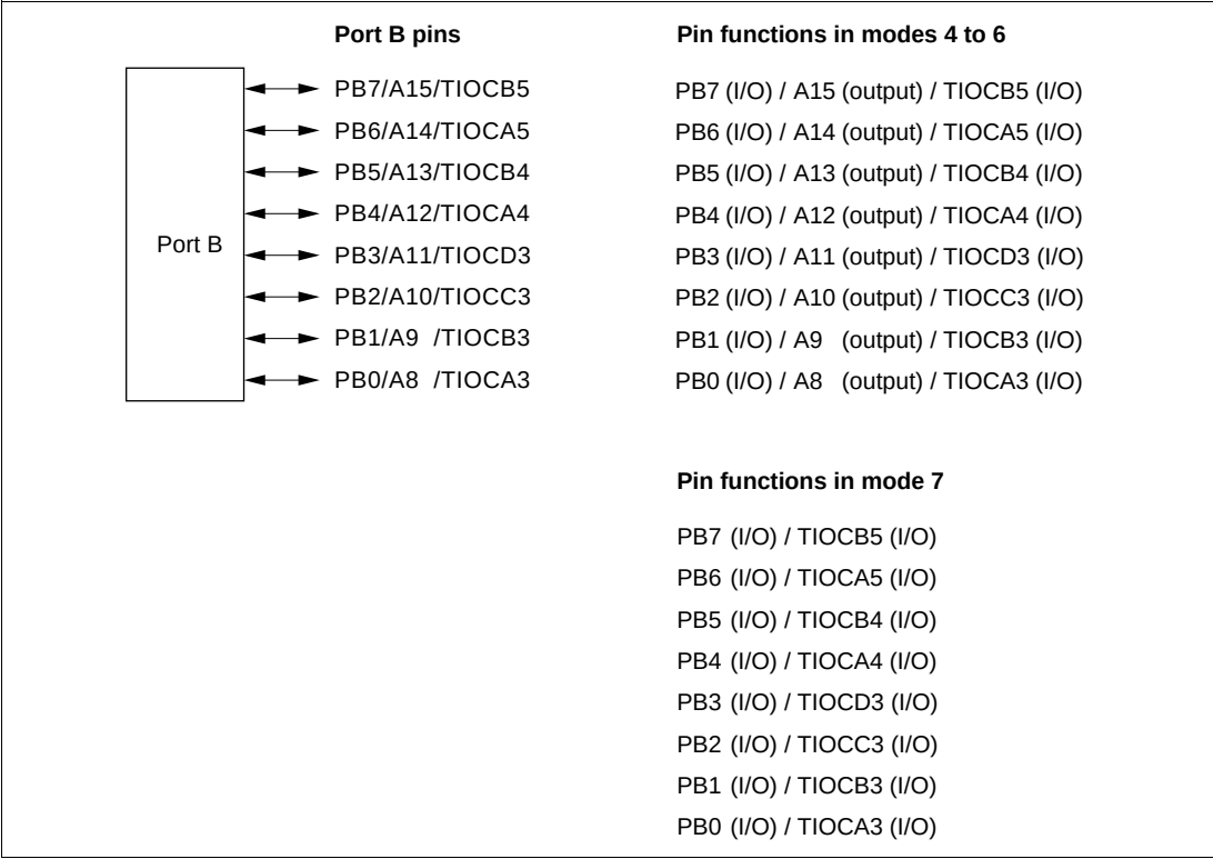
Figure 10B-9 Port B Pin Functions
