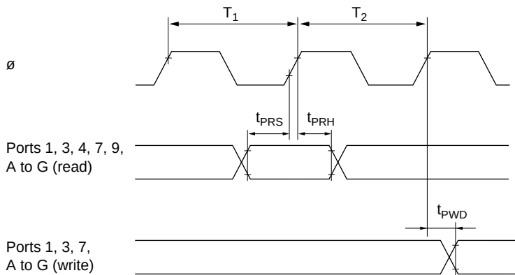
Figure 25-20 I/O Port Input/Output Timing
