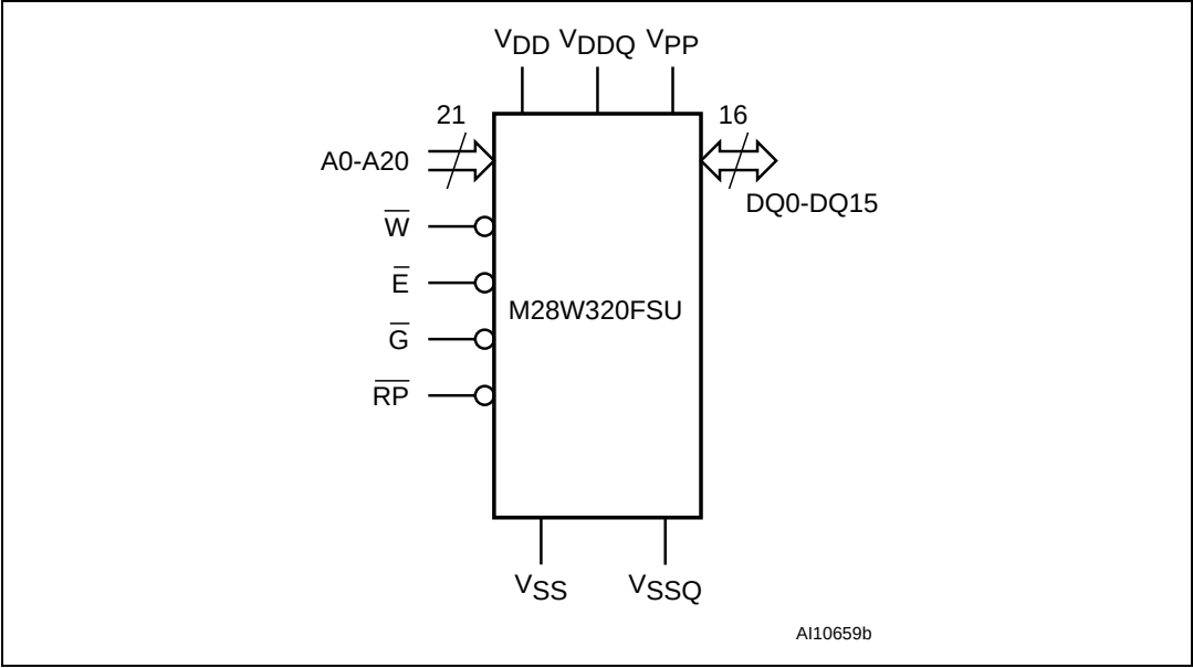
Figure 3. M28W320FSU logic diagram
