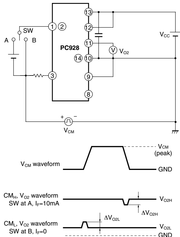
Fig.7 Test Circuit for Instantaneous Common Mode Rejection Voltage
