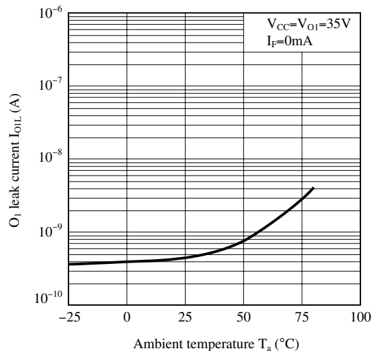
Fig.22 O 1 Leak Current vs. Ambient Temperature
