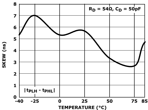
FIGURE 14. DRIVER DIFFERENTIAL SKEW vs TEMPERATURE (ISL31470E, ISL31472E)
