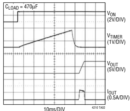
Power-Up Sequence
