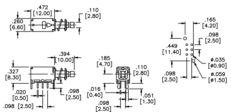
MECHANICAL OUTLINE
