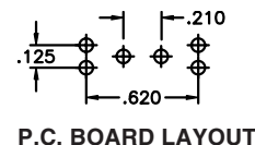
P.C. BOARD LAYOUT
