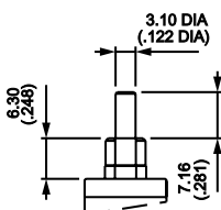
0000 Standard actuator w/smooth bushing
