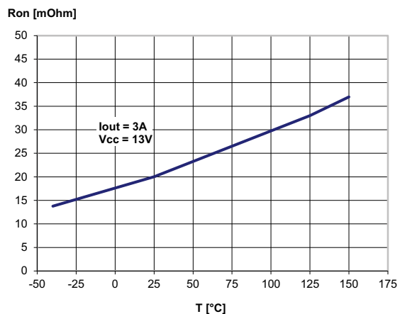
Figure 25. On-state resistance vs. T_{case}
