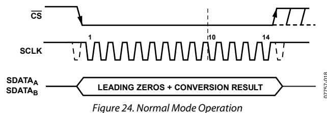
Figure 24. Normal Mode Operation
