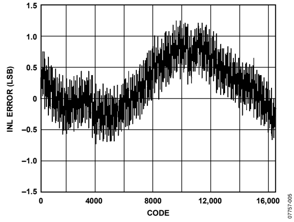
Figure 5. Typical INL
