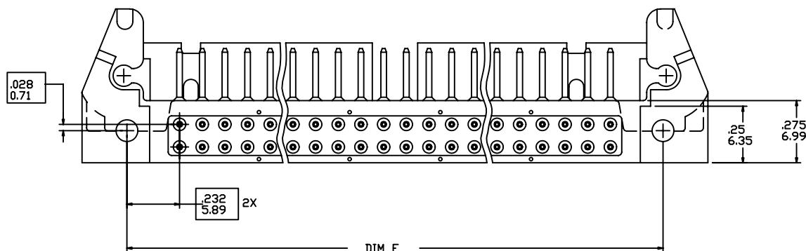
VIEW F-F
