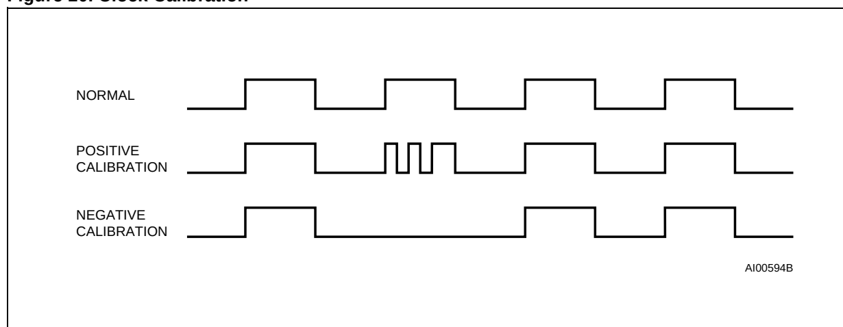
Figure 10. Clock Calibration
