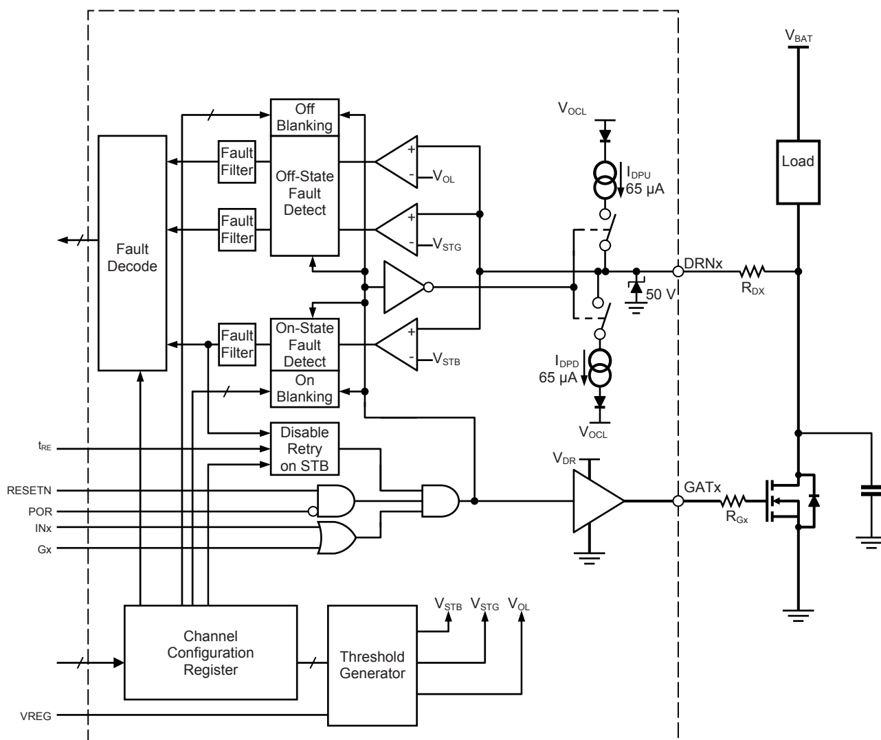
Figure 1. Gate Drive Channel functional block diagram (shows 1 channel of 6)
