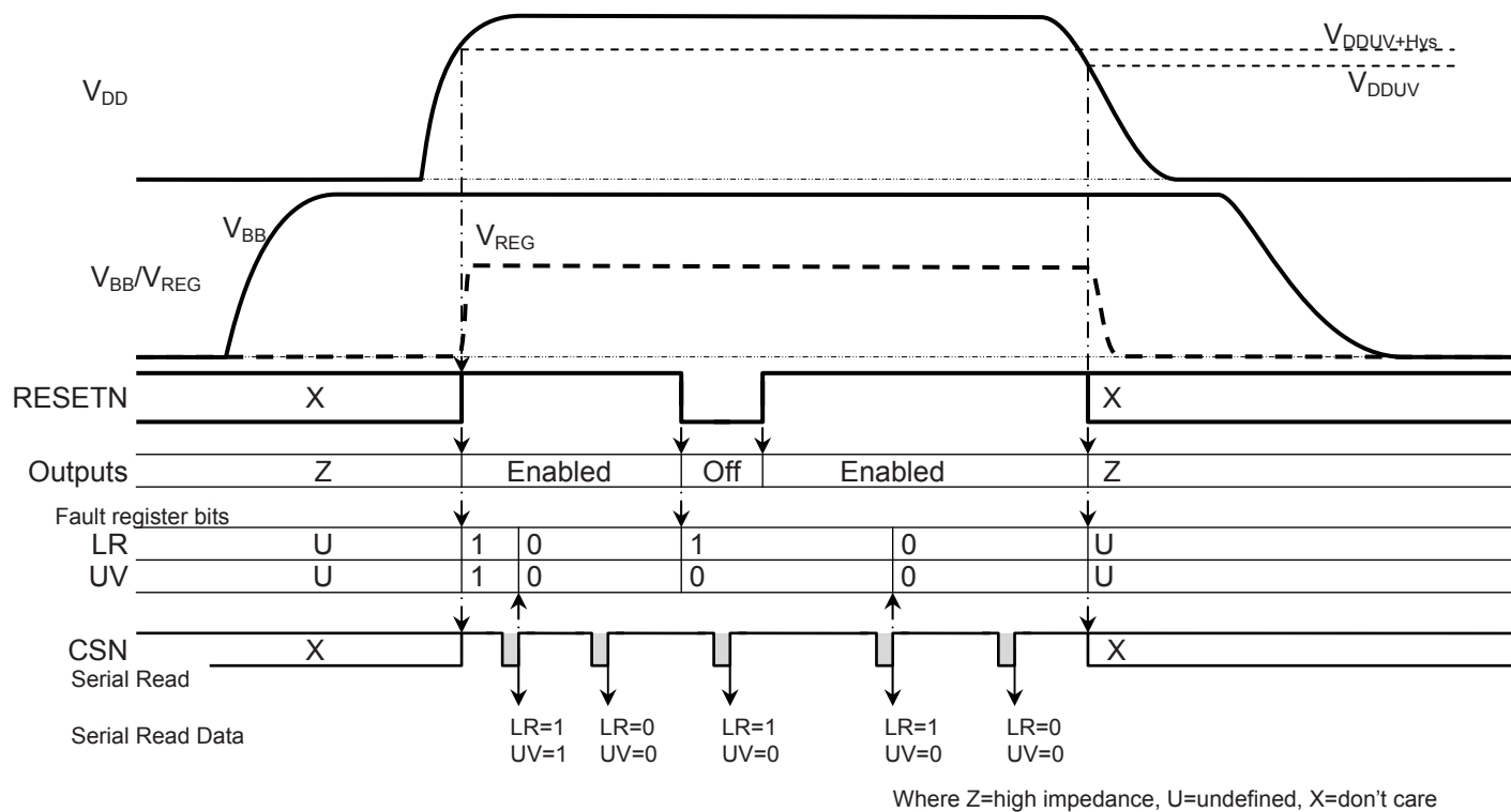
Figure 12. Power Sequence Timing- V_{DD} after V_{BB} - with RESET
