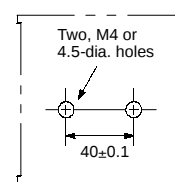
Mounting Holes
