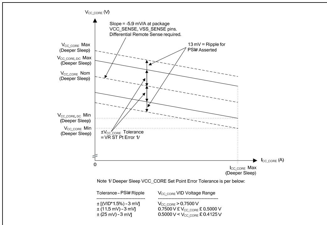
Figure 4. Deeper Sleep VCC and ICC Processor Loadline
