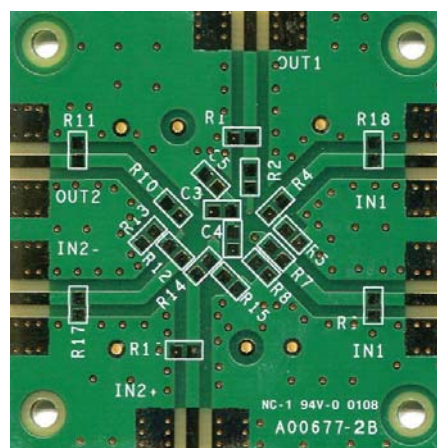
Figure 2. EB-O8RJ-2Z Circuit Side of Evaluation Board
