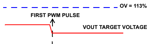
FIGURE 16. SOFT-START WITH VOUT BELOW OV BUT ABOVE FINAL TARGET VOLTAGE
