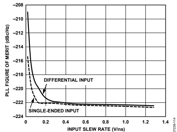
Figure 11. PLL Figure of Merit (FOM) vs. Slew Rate at \overline{REF_{IN}}/\overline{REF_{IN}}
