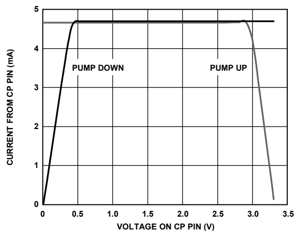
Figure 8. Charge Pump Characteristics at C_P = 3.3 V
