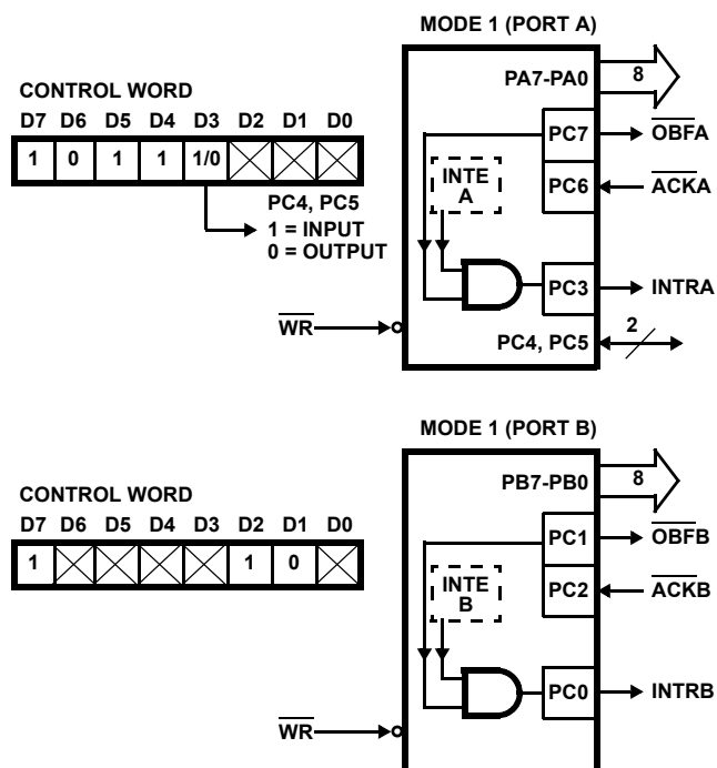
FIGURE 8. MODE 1 OUTPUT
