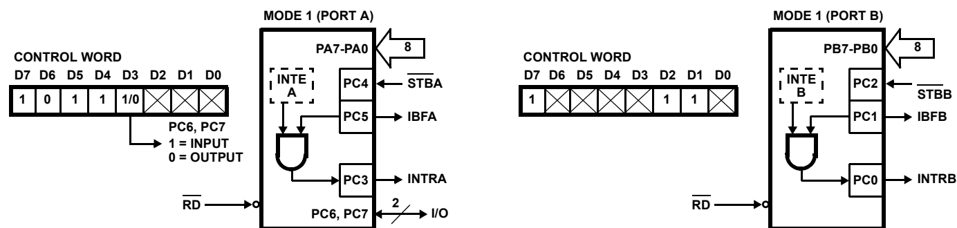
FIGURE 6. MODE 1 INPUT
