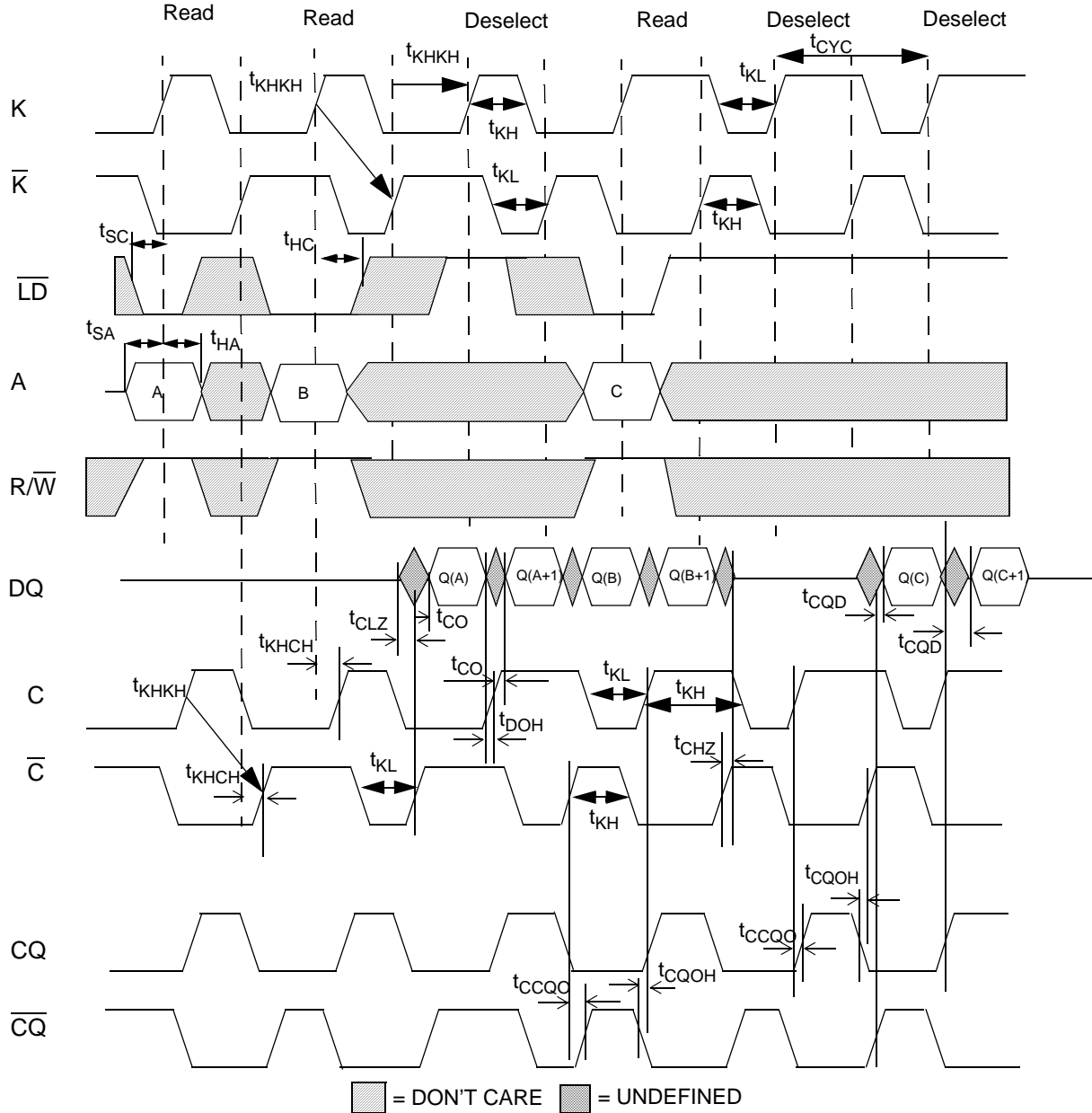
Read/Deselect Sequence [18]
