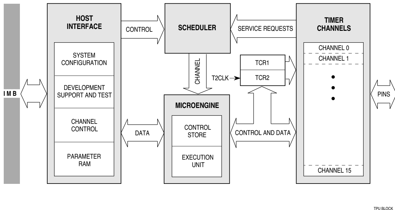
Figure 12 TPU Block Diagram
